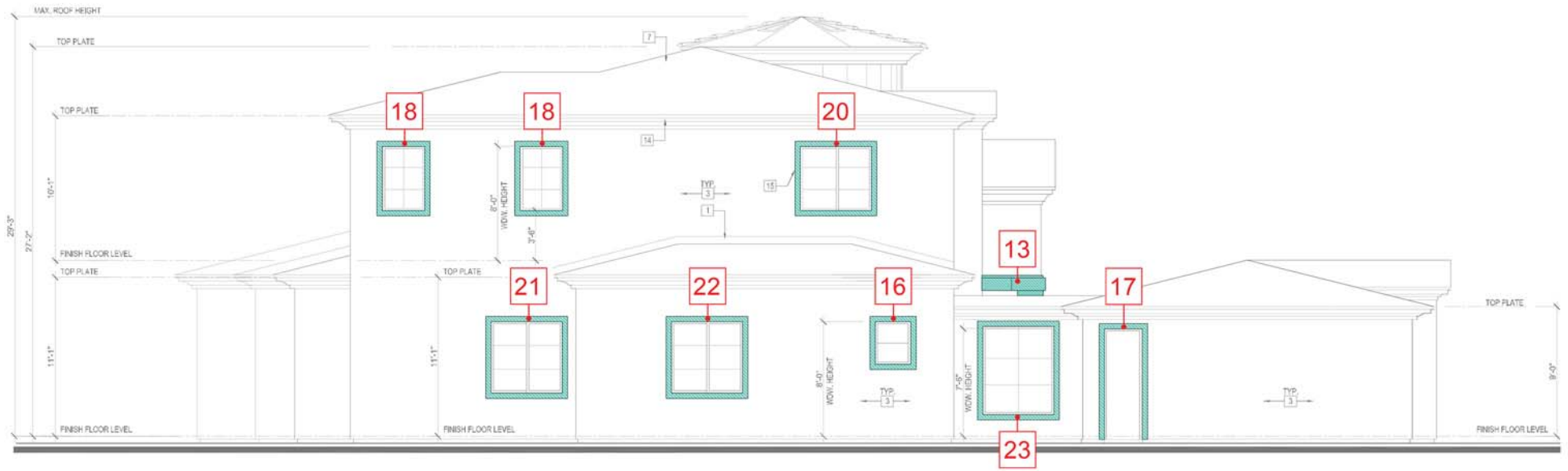
LEFT ELEVATION
