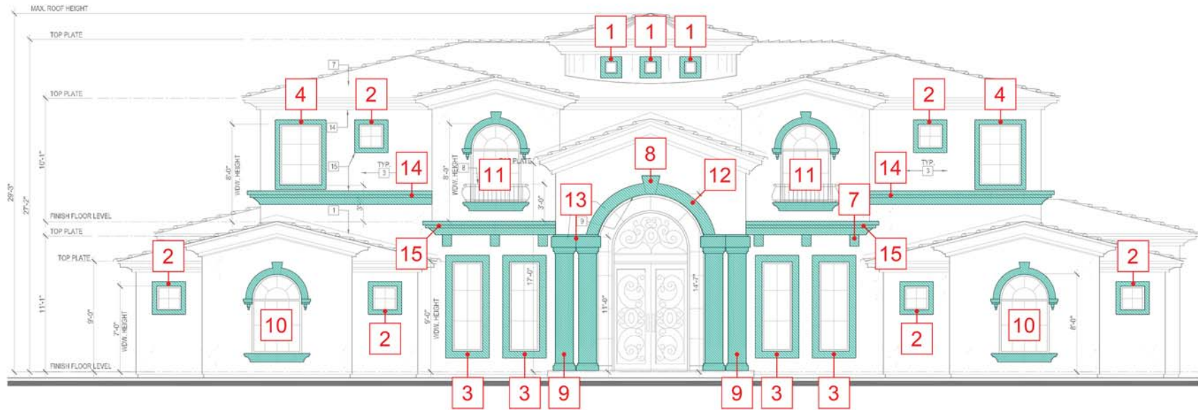
FRONT ELEVATION
